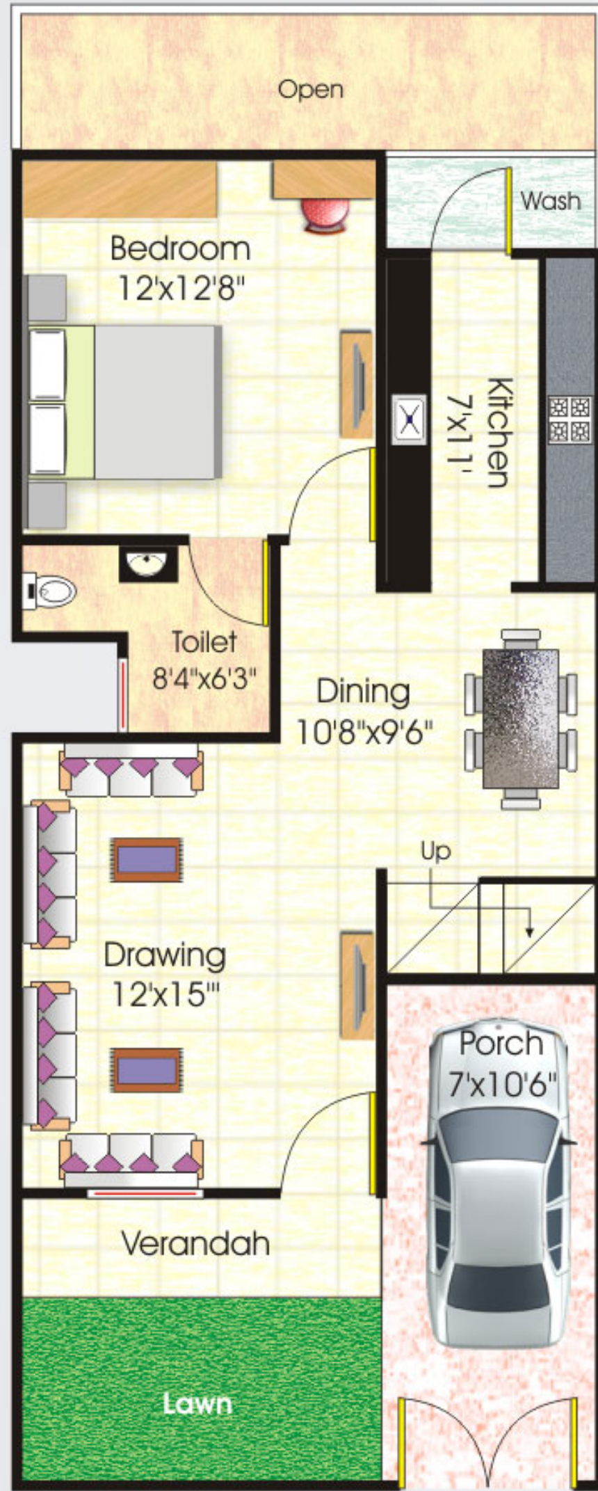
GROUND FLOOR
