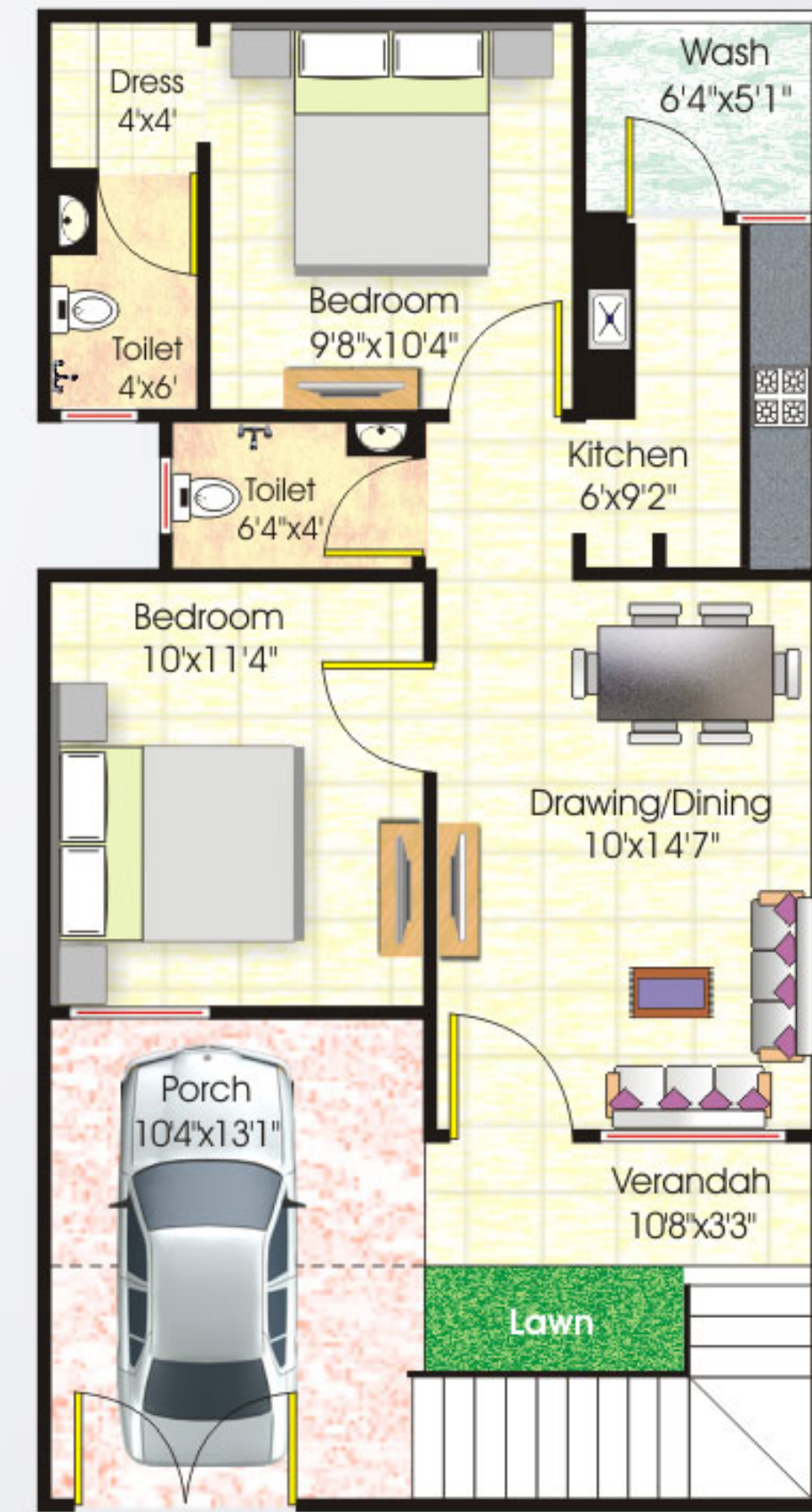
FLOOR PLAN
